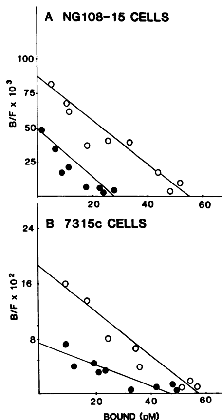
Fig. 2. Scatchard transformation of [ 3 H]ET binding to \delta -receptors in NG108-15 cells (A) or \mu -receptors in 7315c cells (B) suspended in modified Krebs-HEPES buffer. Specific binding was measured at increasing radioligand concentrations from 0.05 to 25 nM, in the presence of 118 mM sodium ( \bullet ), or after equimolar replacement of sodium by N-MG ( \circ ). Data are mean values of triplicate determinations in single experiments, which were each replicated twice with similar results. Estimates of K_D and B_{max} from the combined experiments are listed in Table 1. A, 160 \mu g of protein/assay tube, in the presence and absence of sodium; B, 240 \mu g of protein/assay tube in the presence of sodium, 300 \mu g of protein/assay tube in the absence of sodium. Other details of the incubation conditions are described under Materials and Methods.
