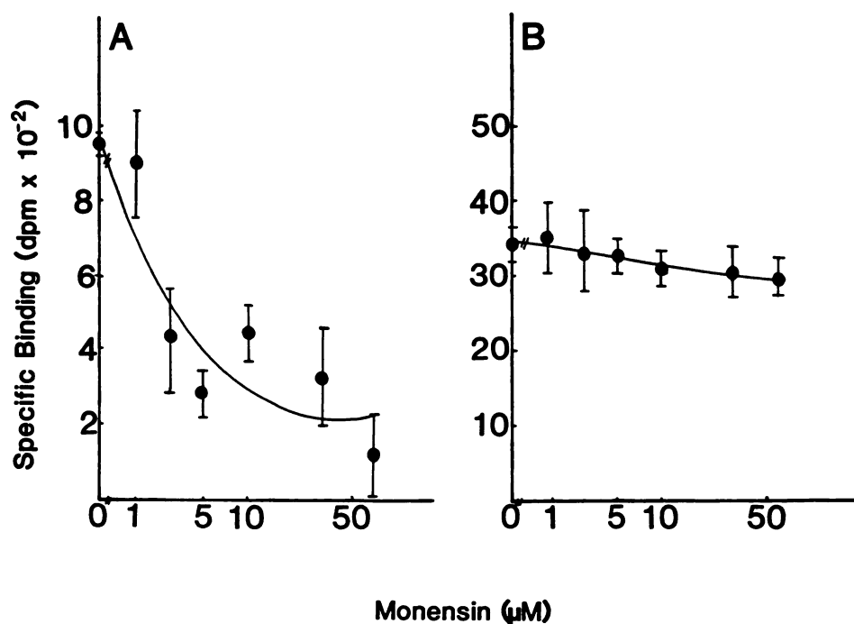
Fig. 4. Effects of monensin on the specific binding of [ 3 H]ET, 2 nM, by \delta -receptors in NG108-15 cells: A, in modified Krebs-HEPES buffer containing 118 mM sodium; B, in modified Krebs-HEPES in which sodium was replaced by an equimolar concentration of N-MG. Results are the mean \pm SE of triplicate determinations. Replicate experiments yielded similar results.
