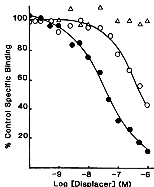
Fig. 3. Inhibition by opioids of specific binding of [ ^3 H]ET, 2 nM, by 7315c membranes. Nonspecific binding was estimated in the presence of 1 \mu M levallorphan. Points are the mean values of triplicate determinations: ●, DADLE; ○, DSLET; △, U50488H.
